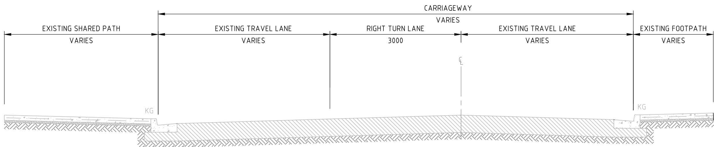
TYPICAL SECTION WILSONS ROAD SECTION 1 SCALE 1:50
